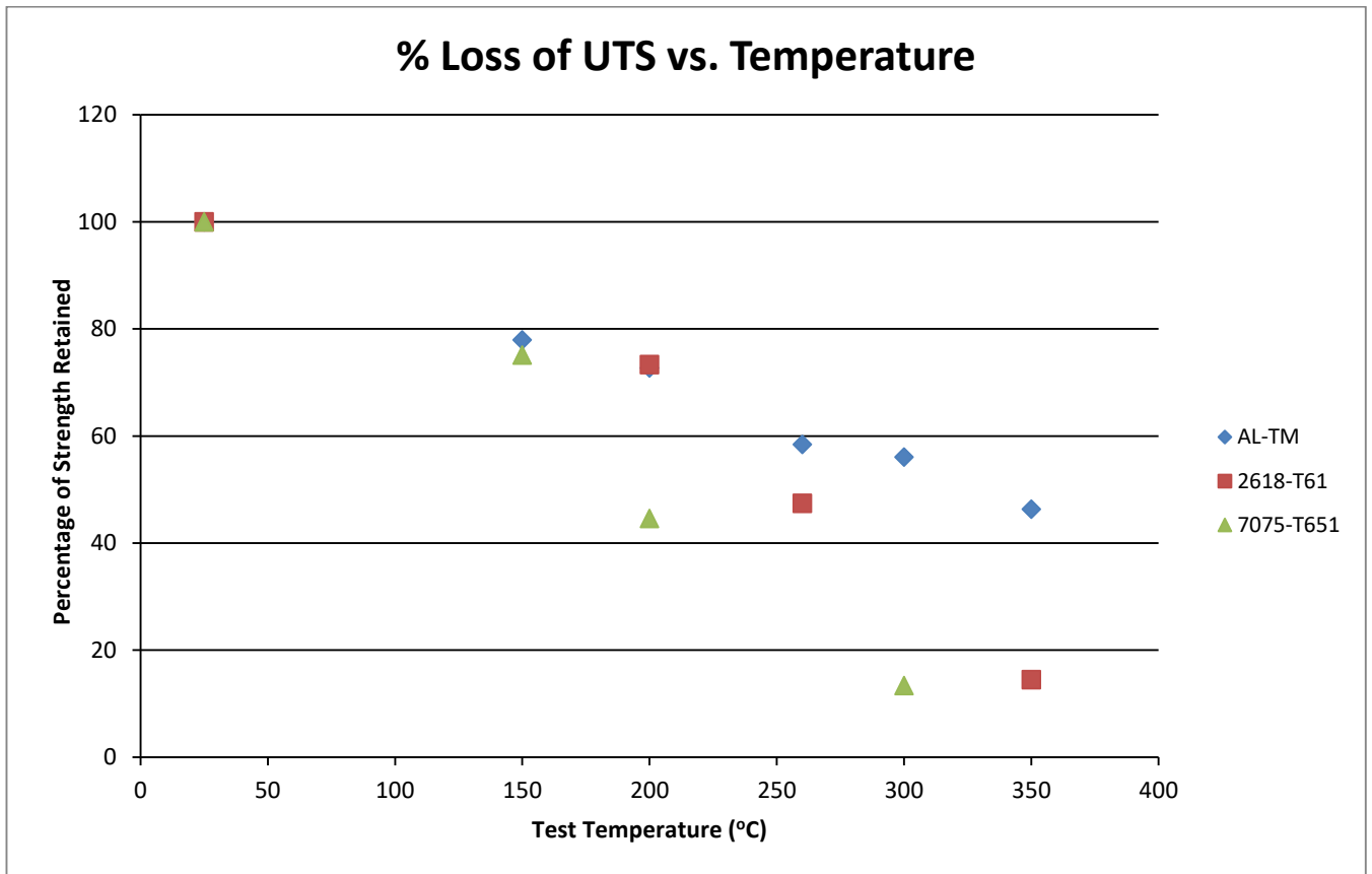
FIGURE [4] / Comparison of the loss in mechanical strength of the AL-12.4TM, 2618 and 7075 alloys as a function of temperature
