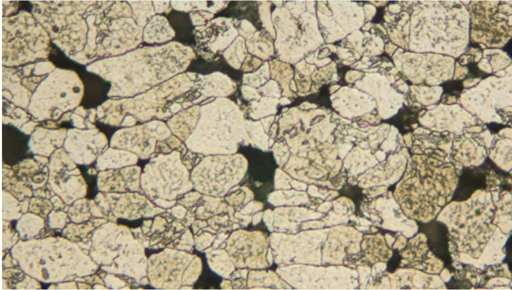
FIGURE [3] / Microstructure of 2000-series aluminum alloy pressed to 2.5 g/cm 3 and sintered at 590°C (1095°F) for 20 minutes in dry nitrogen
