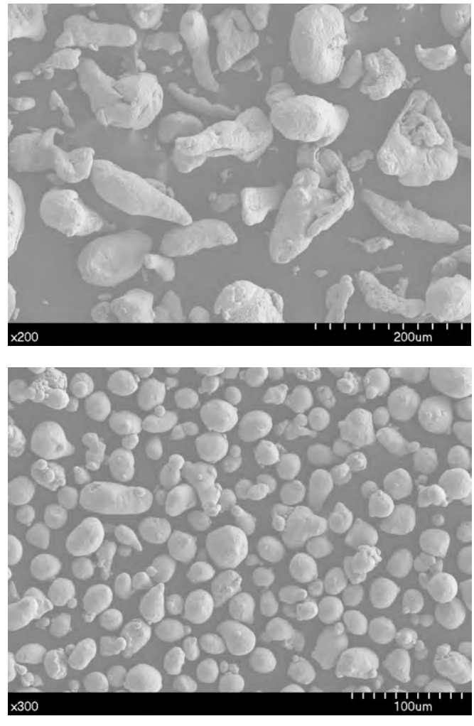
FIGURE [2] / Examples of particle-shape options for aluminum powder
