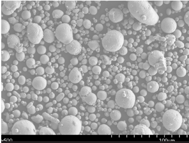
FIGURE [5] / Example of aluminum powder for additive manufacturing
